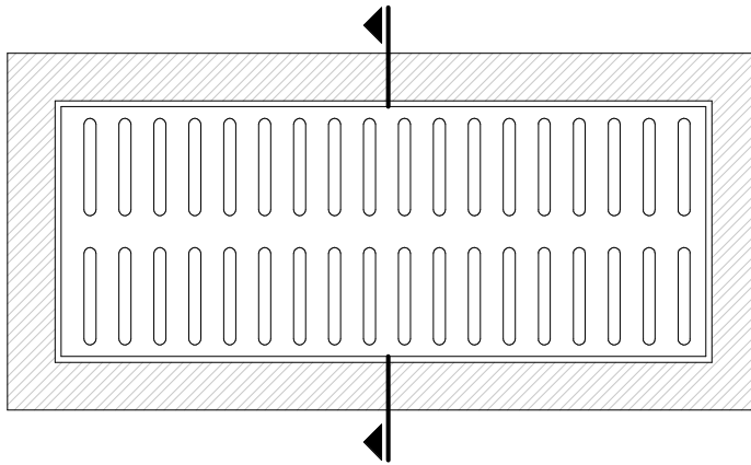
TRENCH DRAIN PLAN VIEW
