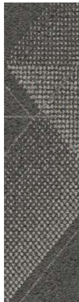
107154 Phosphorus
