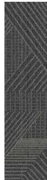
107190 Nitrogen
