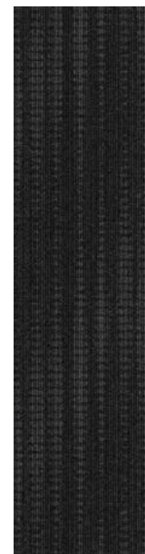
107215 Carbon
