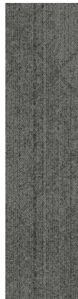
107207 Phosphorus
