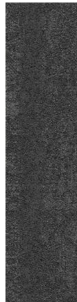
107167 Nitrogen
