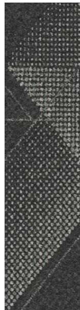
107155 Nitrogen
