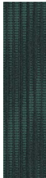
107213 Chromium
