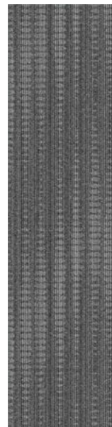
107211 Oxygen
